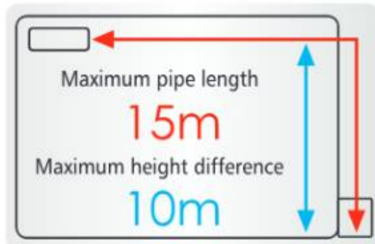
SRK20CSS-S6/A
